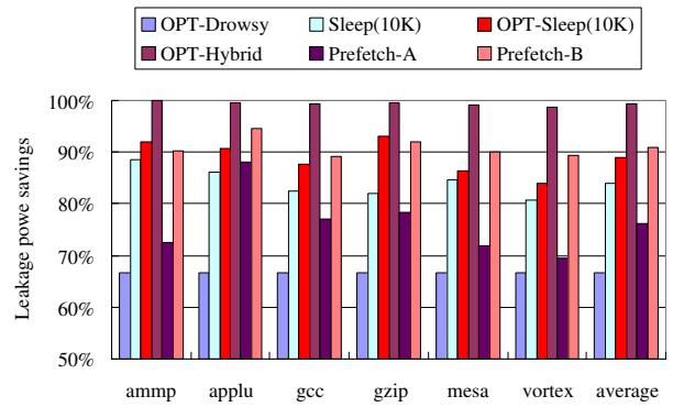
(b) Data Cache
