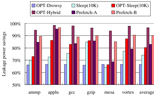
(a) Instruction Cache
